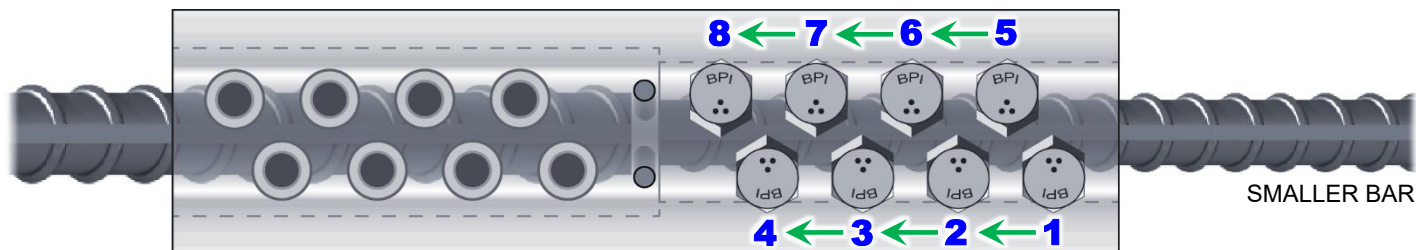
FIGURE 4. Correct Tightening Order, 2 nd Side (#14/10 Transition shown, other sizes similar)
