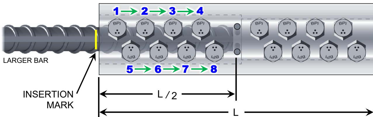
FIGURE 3: Correct Tightening Order, 1 ST Side (#14/10 Transition shown, other sizes similar)
